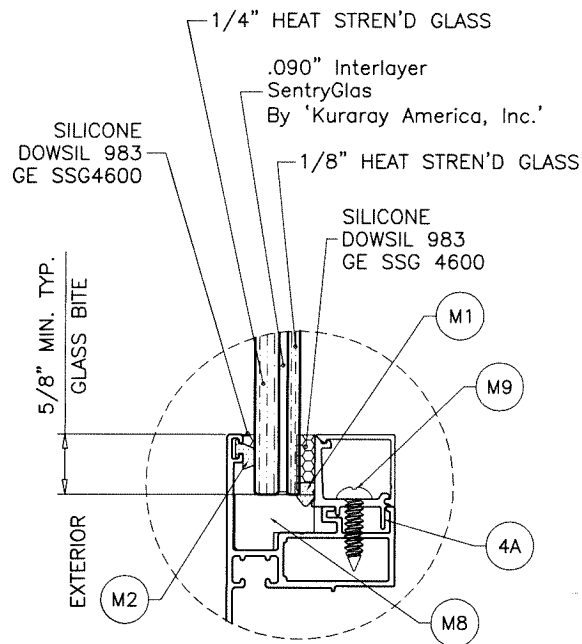
GLASS TYPE 'B' 7/16" OVERALL LAM. GLASS
